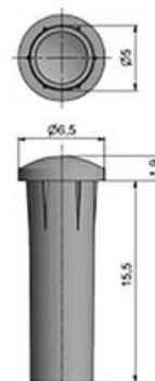
Lightpoint pin O16.1
